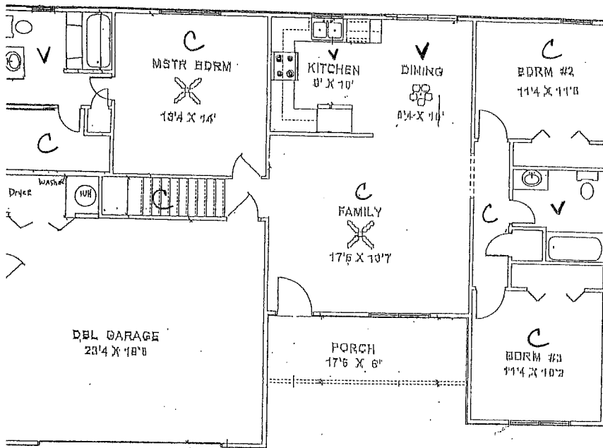
1 st Floor
