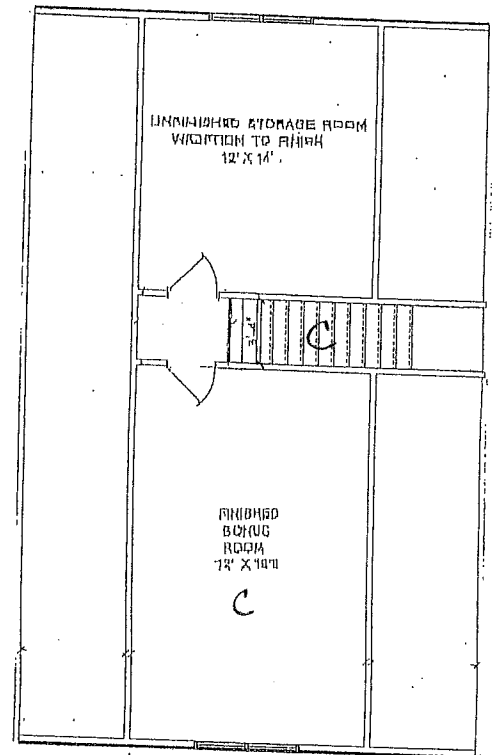
2 nd Floor
