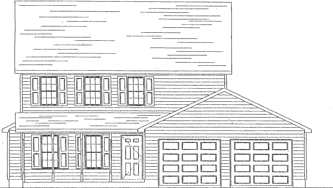
FRONT ELEVATION
